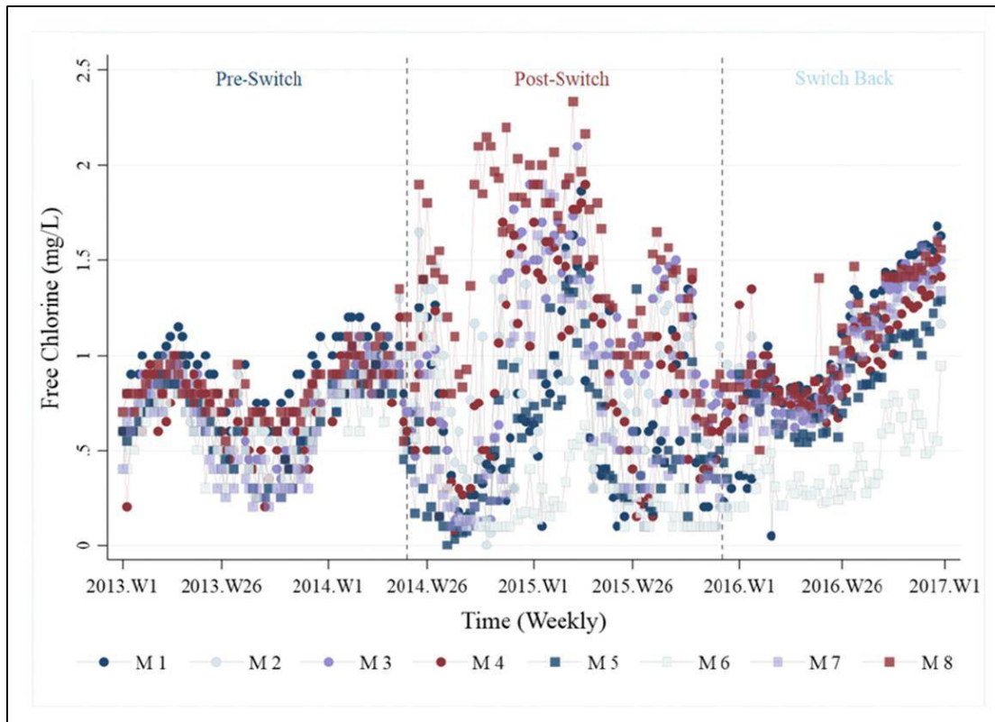
Figure 1: The graph above highlights free chlorine levels from 2013-2016 at eight monitoring stations in Flint’s water distribution system. Adapted from “Assessment of the Legionnaires’ disease outbreak in Flint, Michigan” Zahran, S, et al. 2018 PNAS February 5, 2018. Page E1731. Copyright 2018, National Academy of Sciences.
